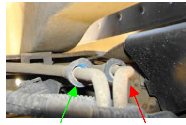
Suction Line Return Line Figure 27
