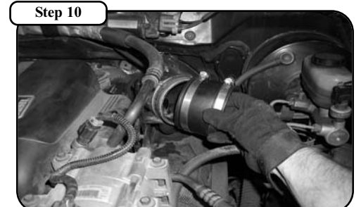
Place provided clamps loosely over provided coupler and place onto factory turbo inlet elbow
