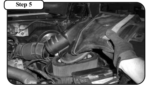
Remove top half of air box from lower half. Remove factory intake tube from factory turbo inlet elbow.
