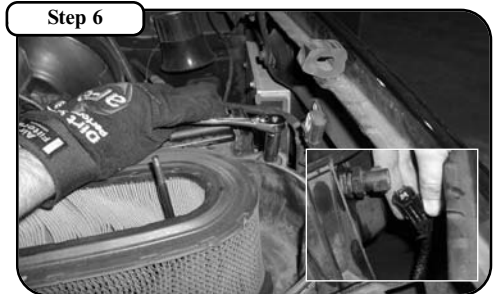
Using a 7/16" socket, remove nut securing lower air box half to engine compartment. Disconnect electrical harness going to temperature sensor on the side of the air box.
