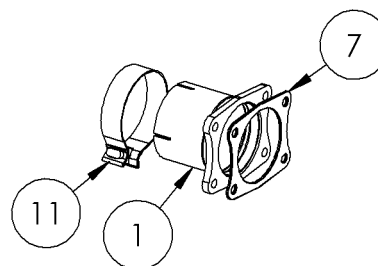
DETAIL B SCALE 1 : 10
