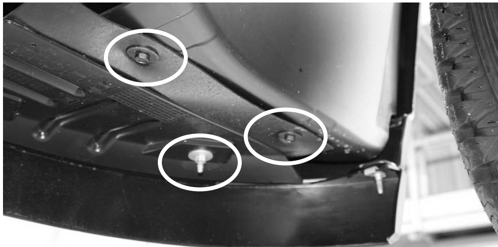
Figure 1 - Screw Locations
