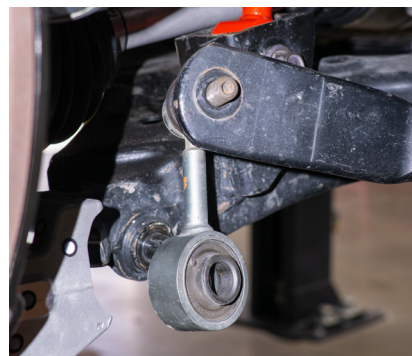
Fig. 2: Sway bar end link.
