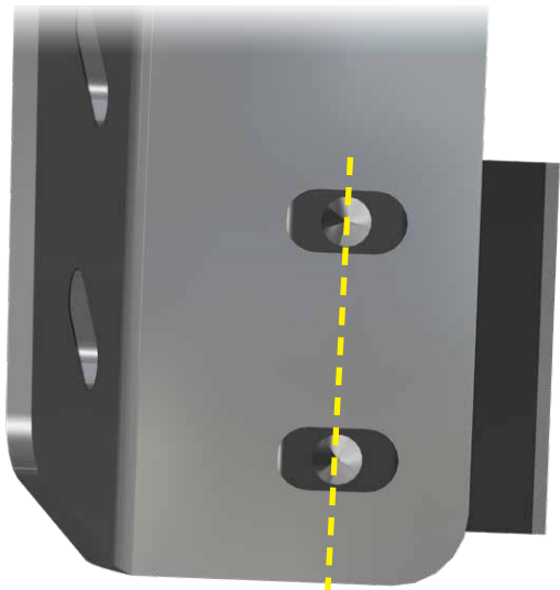
center slots on Clamps
