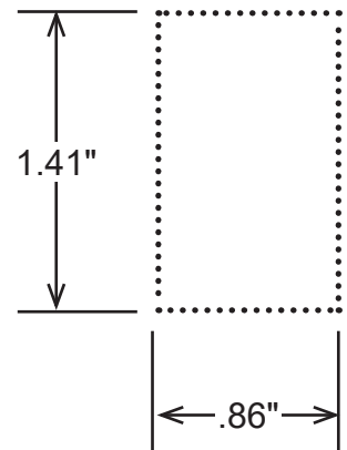
Mounting Slot:
