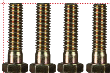
FOUR (4) HEX BOLT 3/8"-16x11/2"
