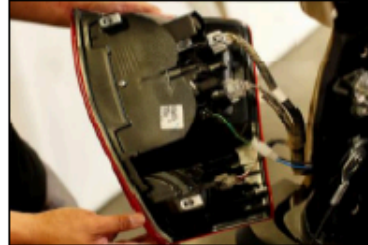
Connect 3 factory connections and resistor connection to Anzo USA tail light.
