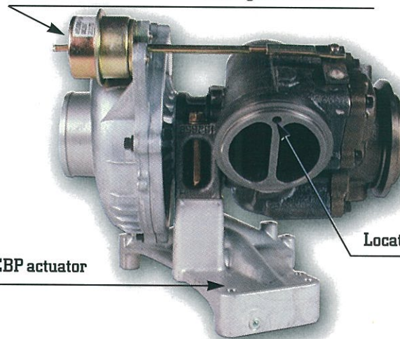
Wastegate actuator
