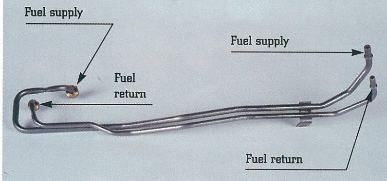
Fuel filter to chassis connections
