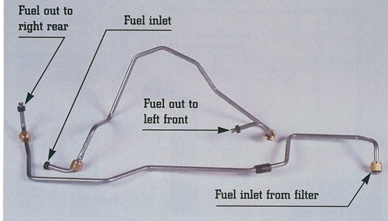
Fuel filter to chassis connections
