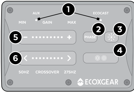
CONTROL PANEL
