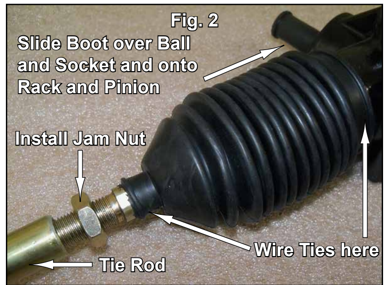
(Rack and Pinion shown off machine for clarity)
