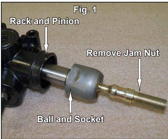
(Rack and Pinion shown off machine for clarity)
