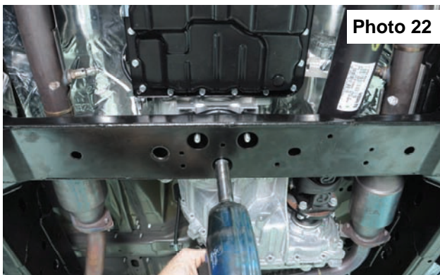
Remove transmission mount nuts.
