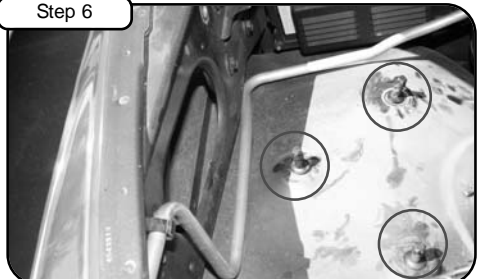
Remove plastic fittings from bolts on existing stock location mounts. Make sure 1/4-20" screw is showing.
