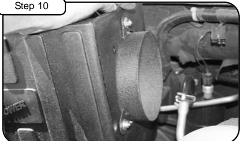
Install filter adaptor to outside of housing using supplied screws, washers, and nuts. Tighten with 7/16" socket or wrench.
